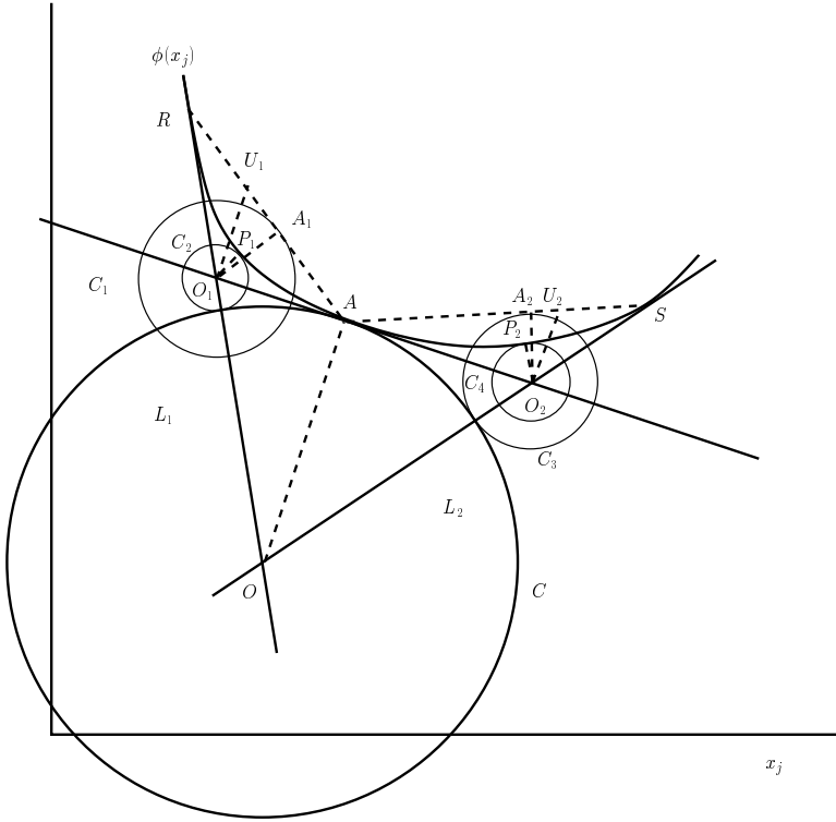
Fig. 2. Proof of Theorem 3.
